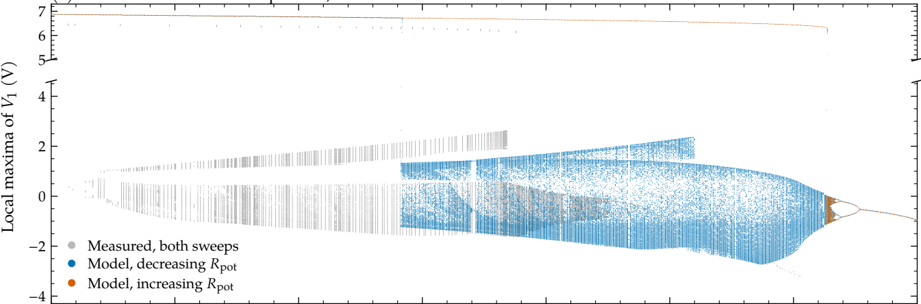
(a) Ideal model: nominal components, element of Table 2
